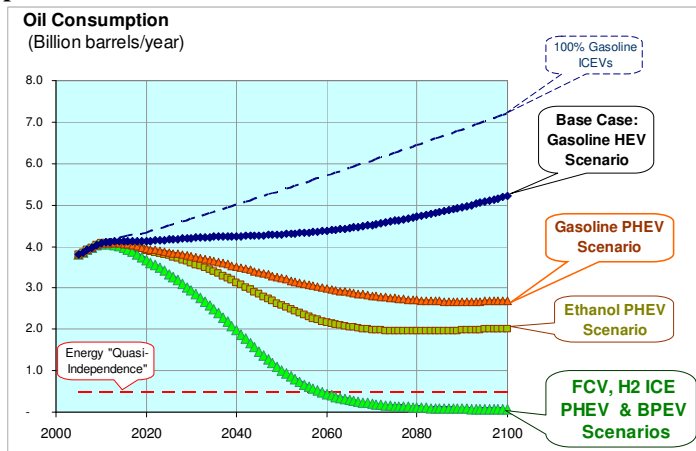
Figure 3. Petroleum consumption projections for the alternative vehicle scenarios, including the estimated oil consumption level such that US domestic production could supply all non-transportation petroleum requirements.
