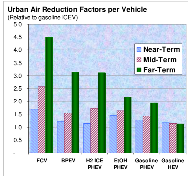
Figure 17. Urban air pollution reduction factors relative to gasoline ICEVs
