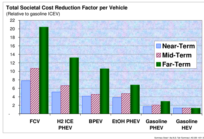
Figure 7. Societal cost reduction factors for alternative vehicle/fuel combinations over three time periods: near-term (now to 2020), mid-term (2021 to 2050) and far-term (2051 to 2100)
