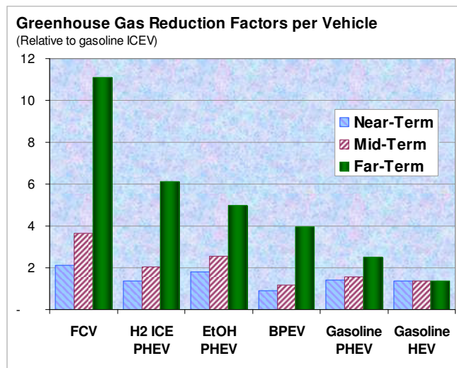
Figure 16. Greenhouse gas reduction factors compared to gasoline ICEVs
