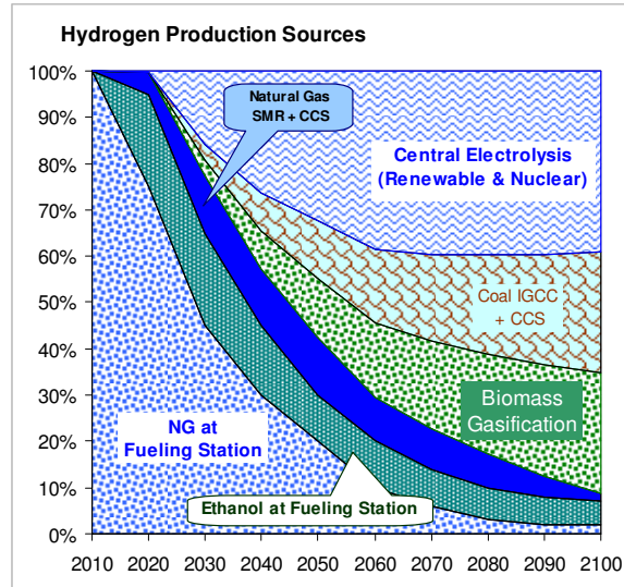
Figure 14. Postulated sources of hydrogen over time
